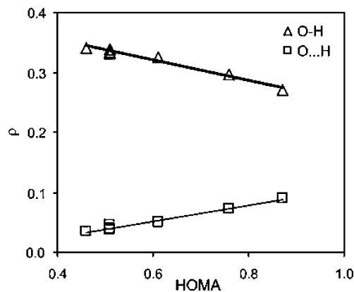
Figure 37. Dependences of electron density in BCP of O–H bond ( \Delta ) and O \cdots H bond ( \square ) on HOMA values for substituted derivatives of malonaldehyde. Correlation coefficients are -0.989 and 0.990 , respectively. Reprinted with permission from (Krygowski, T. M.; Zachara, J. E., Theor. Chem. Acc. , in press), copyright Springer, New York.
