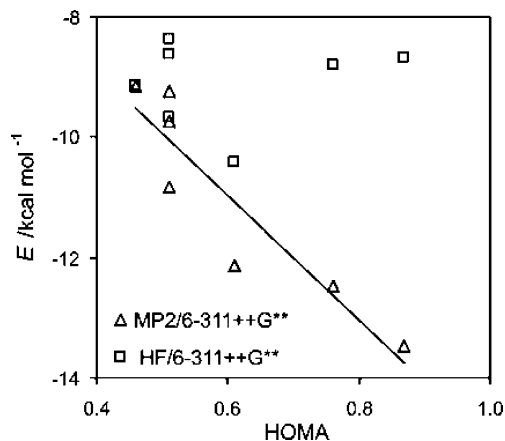
Figure 39. Dependence of H-bond energy on HOMA values for two levels of theory employed: HF/6-311++G(d,p) (□) and including the electron correlation, MP2/6-311++G(d,p) (Δ). Correlation coefficient for the latest relationship -0.920 . Reprinted with permission from (Krygowski, T. M.; Zachara, J. E., Theor. Chem. Acc. , in press), copyright Springer, New York.
