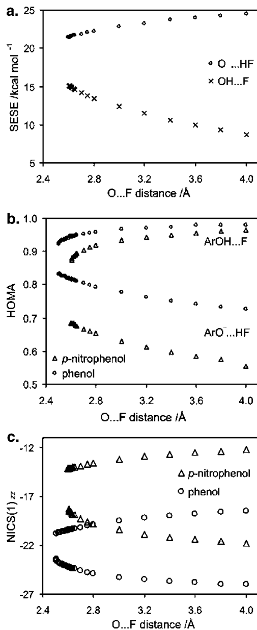
Figure 30. (a) Scatter plots of SESE values (Chart 25) for two kinds of H-bond (eqs 25a and 25b) versus the O\cdots F distance. Variation of (b) HOMA values and (c) NICS (1)_{zz} values for ArOH\cdots F^- and ArO^-\cdots HF interactions for p -nitrophenol ( \Delta ) and phenol ( \circ ) complexes. Reprinted with permission from (Krygowski, T. M.; Zachara, J. E.; Szatyłowicz H. J. Org. Chem. 2004 , 69 , 7038), copyright 2004, American Chemical Society, Washington, DC.
