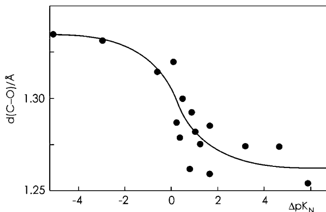
Figure 9. Correlation between the C–O bond length and \Delta pK_N for complexes of pentachlorophenol and 2,6-dichloro-4-nitrophenol. Reprinted with permission from (Majerz, I.; Malarski, Z.; Sobczyk, L. Chem. Phys. Lett. 1997 , 274 , 361), copyright 2004, Elsevier, Amsterdam, The Netherlands.
