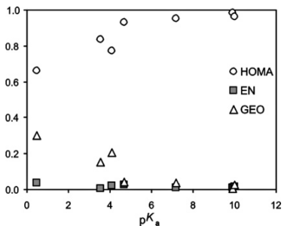
Figure 26. Plot of HOMA, GEO, and EN mean values versus pK_a for seven types of substituted phenol. Reprinted with permission from (Krygowski, T. M.; Szatyłowicz H.; Zachara J. E. J. Chem. Inf. Comput. Sci. 2004 , 44 , 2077), copyright 2004, American Chemical Society, Washington, DC.
