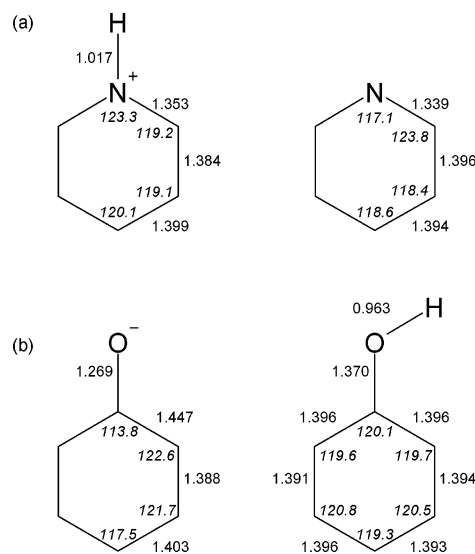
Figure 35. Bond lengths (Å) and bond angles (deg) of pyridine and pyridinium cation (Majerz, I.; Koll, A. Acta Crystallogr., Sect. B: Struct. Sci. 2004 , 60 , 406) and of phenol and phenolate (Szatyłowicz, H.; Zachara, J. E., private communication).
