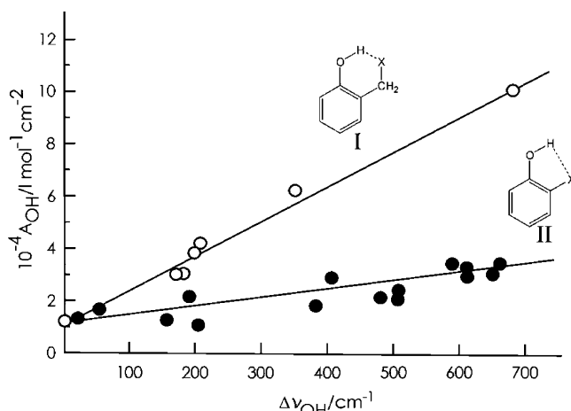
Figure 11. Integrated intensity of the \nu_{\text{OH}} band plotted versus frequency shift \Delta\nu_{\text{OH}} for two types of intramolecular H-bonds: conjugate chelate (II) and isolated (I). Reprinted with permission from (Takasuka, M.; Matsui, Y. J. Chem. Soc., Perkin Trans. 2 1979 , 1743), copyright 2004, Royal Society of Chemistry, London, U.K.
